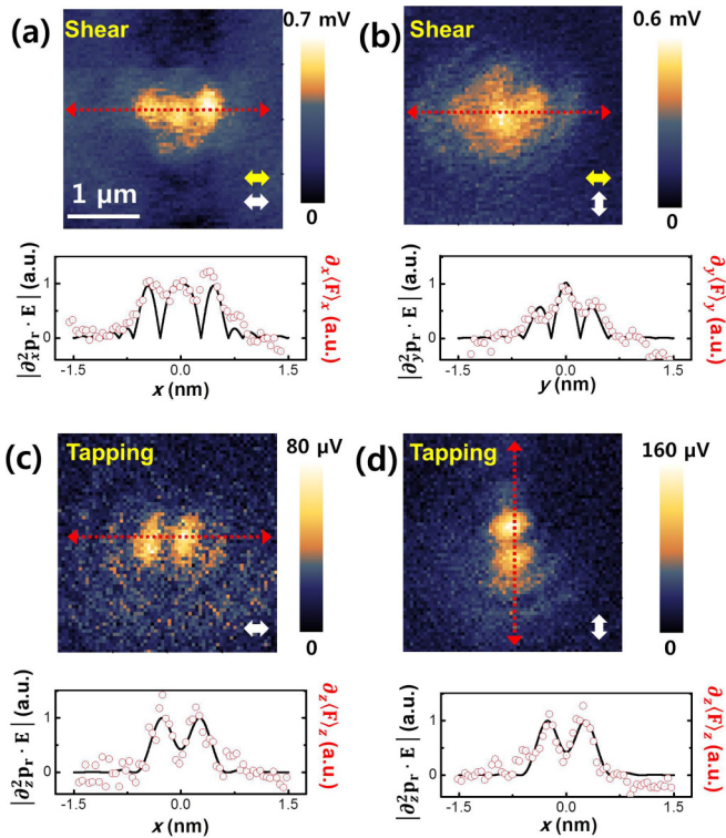
FIG. 7. Measured PiFM amplitude maps of a tightly focused laser beam obtained with the QTF. The image size is 3 \mu\text{m} \times 3 \mu\text{m} . (a, b) The photoinduced force measured in the shear force mode. (c, d) The photoinduced force measured when using the tapping mode. The yellow arrow depicts the oscillating direction of the tip while the white arrow is the electric field polarization direction (assumed to be along the x axis). Red arrows in each panel show the position where cross sections are taken, displayed below each panel. The open red dots in the cross sections show the normalized QTF amplitude ( A_s \propto \partial_s F_s ), which are compared to the simulated values |\partial_i^2 \mathbf{p} \cdot \mathbf{E}| (black solid line) retrieved from Fig. 6.
