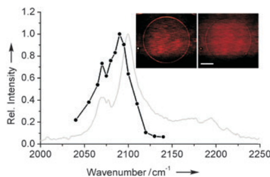
Figure 1. Raman (grey line) and CARS (black dots) spectra of deuterated DSPC ( [D_{70}] DSPC). The CARS spectrum shows a characteristic red-shift relative to the Raman spectrum. In the inset, the left panel shows a CARS image of a [D_{70}] DSPC giant unilamellar vesicle recorded at 2090\text{ cm}^{-1} , the right panel shows the same vesicle imaged at 2140\text{ cm}^{-1} . Images were recorded at room temperature ( 21^\circ\text{C} ). Scale bar is 10\text{ }\mu\text{m} .
