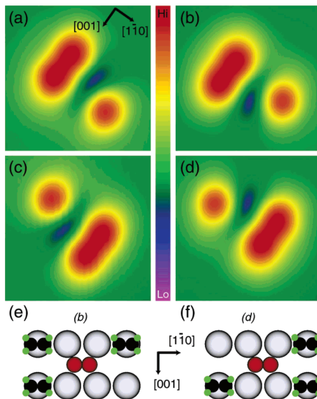
Figure 4. Attachment of a third ethylene to the (C_2H_4)_2-O_2 complex (Figures 2 and 3) to give a three-ethylene complex. The three ethylene molecules can sit on three of the four equivalent nnnt sites to form four (C_2H_4)^{nnnt}_3-O_2(1\bar{1}0) configurations (a–d). (e) and (f) Schematic diagrams for b and d, respectively. The images were obtained with a bare tip at 70 mV sample bias and 1 nA tunneling current. Scan area is 25 \text{ \AA} \times 25 \text{ \AA} .
