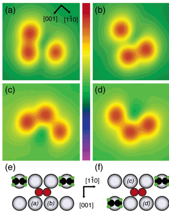
Figure 5. Movement of one ethylene of the (\text{C}_2\text{H}_4)^{\text{nnnt}_3}\text{-O}_2(1\bar{1}0) complex (Figure 4) to a nnt site by 200 meV tunneling electrons gives rise to eight (\text{C}_2\text{H}_4)^{\text{nnnt}_2}\text{-O}_2(1\bar{1}0)\text{-C}_2\text{H}_4^{\text{nnt}} configurations (four shown in a–d). (e) and (f) Schematic diagrams for configurations a–d. The images were obtained with a bare tip at 70 mV sample bias and 1 nA tunneling current. Scan area is 25 \text{ \AA} \times 25 \text{ \AA} .
