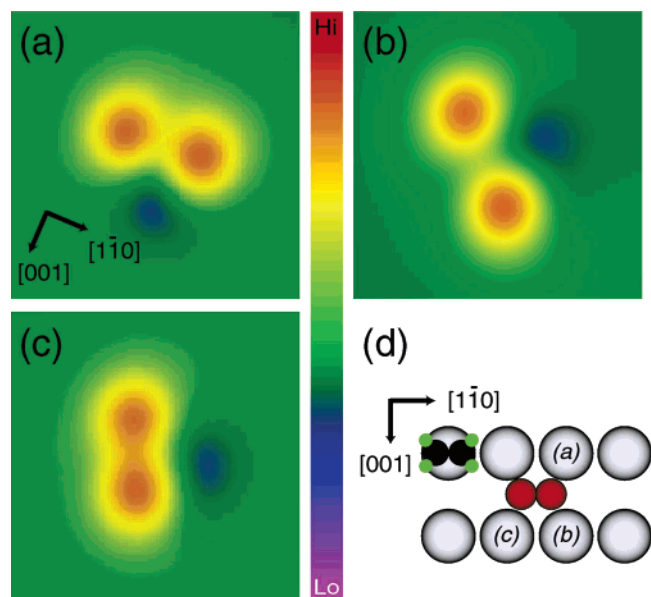
Figure 3. Injection of tunneling electrons ( \sim 200 meV at 1 nA tunneling current) on the C_2H_4 of the (C_2H_4)^{nnnt}_2-O_2(1\bar{1}0) (Figure 2) leads to the formation of different configurations of the two-ethylene complexes. One C_2H_4 moves closer to the O_2(1\bar{1}0) to form the C_2H_4^{nnnt}-O_2(1\bar{1}0)-C_2H_4^{nnt} complexes (a–c). (d) Schematic diagrams for a–c. Twelve configurations were observed for this type of complex. The images were obtained with a bare tip at 70 mV sample bias and 1 nA tunneling current. Scan area is 25 \text{ \AA} \times 25 \text{ \AA} .
