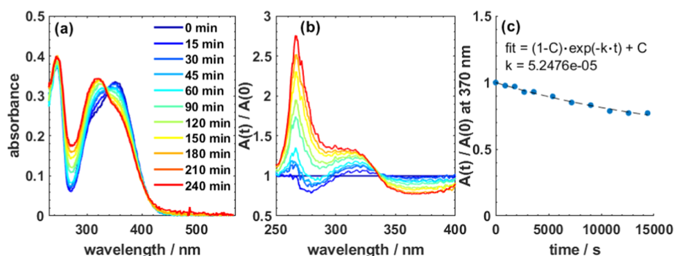
Figure 1. Plot of the absorption spectra of 4NC in isomalt glass obtained at different times during photolysis (a), the same absorbance spectra normalized to the absorbance at t = 0 (b), and the decay in normalized absorbance at 370 nm (c). Notable features of these data are the growth of absorbance at wavelengths below 340 nm and above 400 nm, as well as the decay around the 350 nm band of 4NC.
