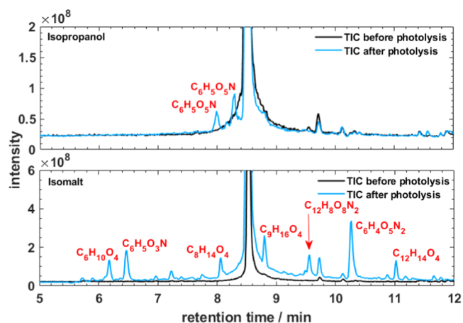
Figure 2. Total ion current chromatograms from UPLC-HRMS analysis of 4-nitrocatechol in isopropanol (top) and 4-nitrocatechol/isomalt glass (bottom) before and after photolysis. Molecular formula assignments are provisional and represent the molecular species eluted at that peak retention time.
