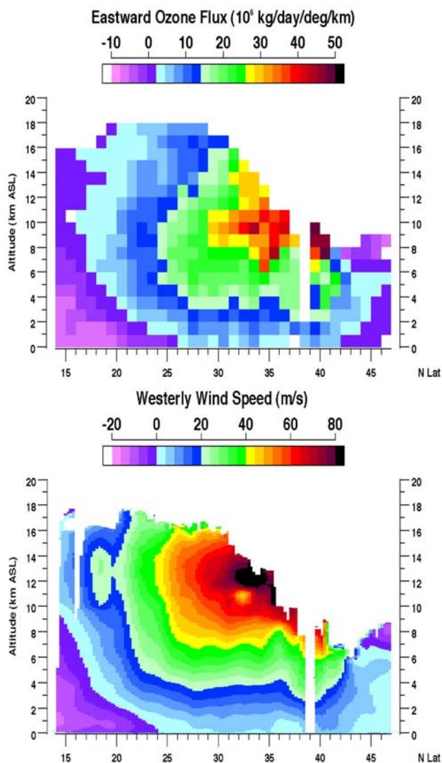
Figure 13. Average latitudinal eastward O_3 flux (top) and westerly wind speed distributions obtained on all TRACE-P flights west of 150^\circ E .
