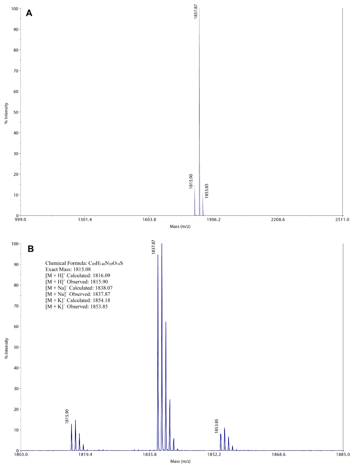
Figure 1.13. MALDI-TOF mass spectrum of peptide 2c . A) Full spectrum. B) Zoomed in spectrum.
