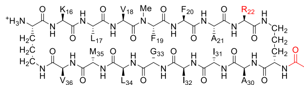
peptides 1c , 2c , 3c
