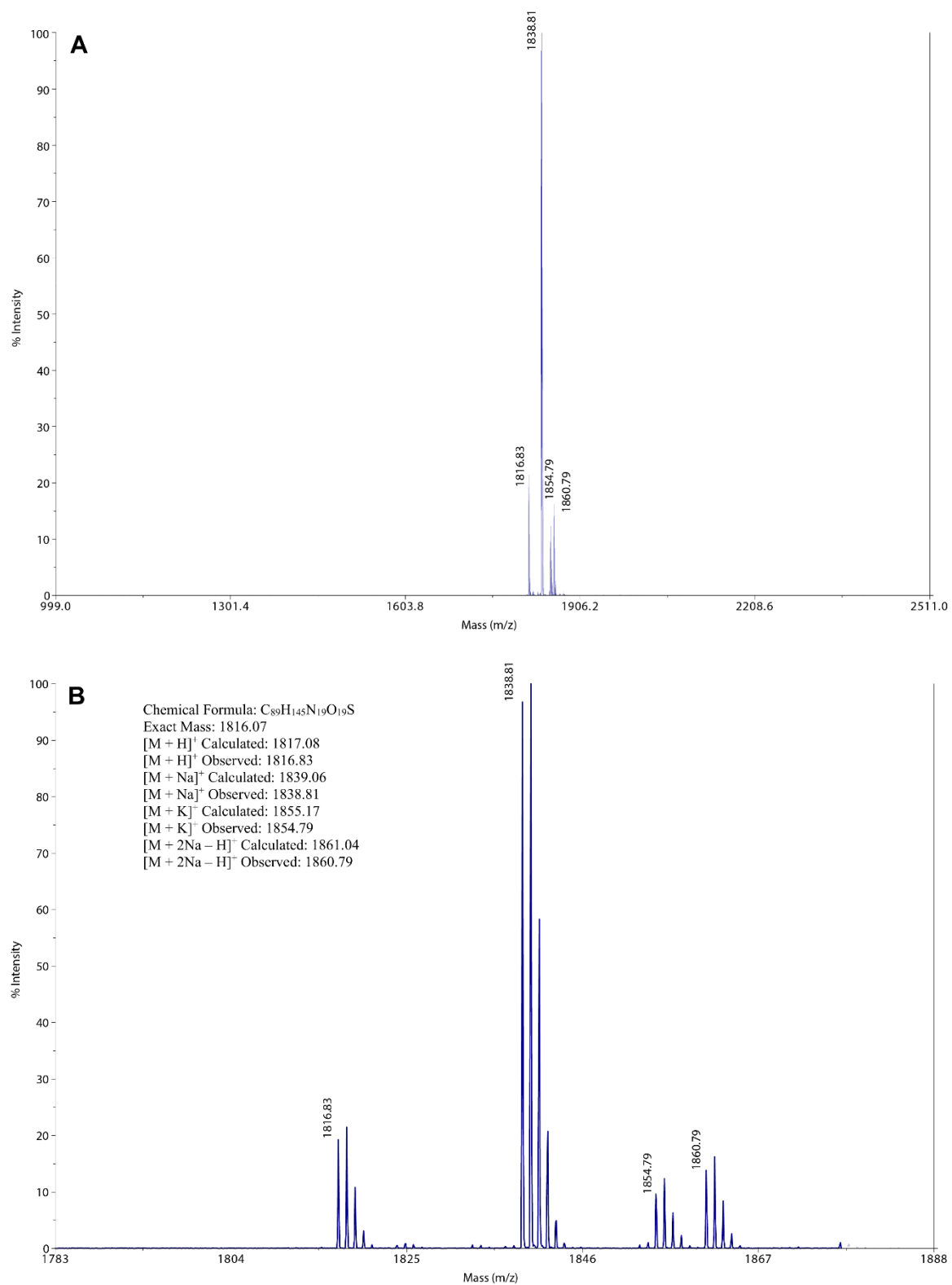
Figure 1.7. MALDI-TOF mass spectrum of peptide 1c . A) Full spectrum. B) Zoomed in spectrum.
