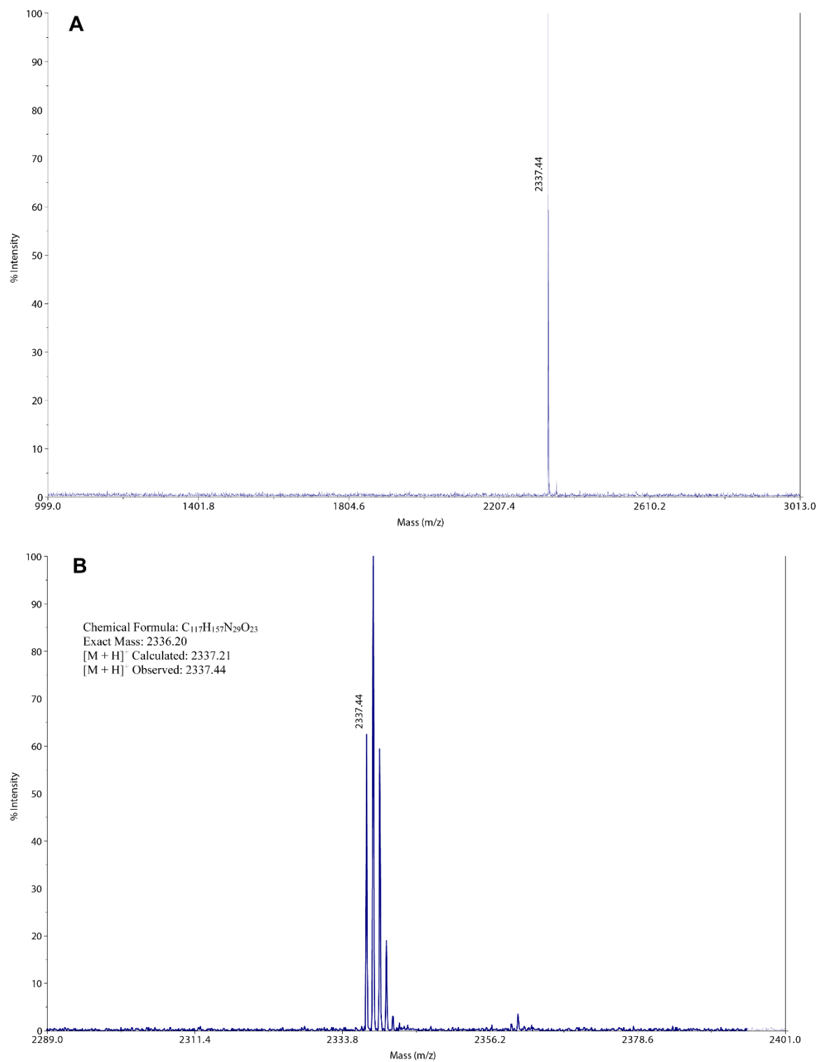
Figure 3.13. MALDI-TOF mass spectra of peptide 2 . A) Full spectrum. B) Zoomed in spectrum.
