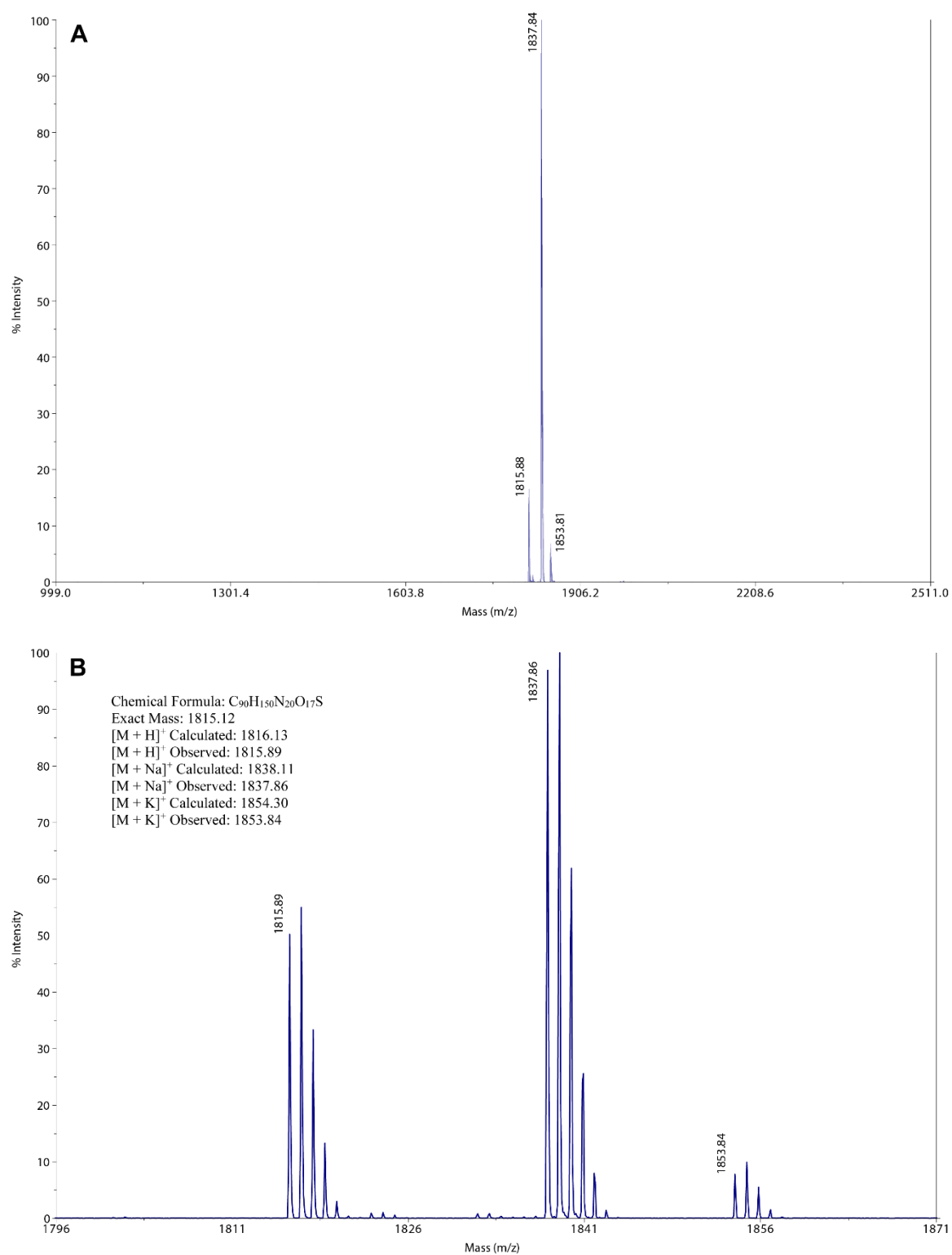
Figure 1.11. MALDI-TOF mass spectrum of peptide 2b . A) Full spectrum. B) Zoomed in spectrum.
