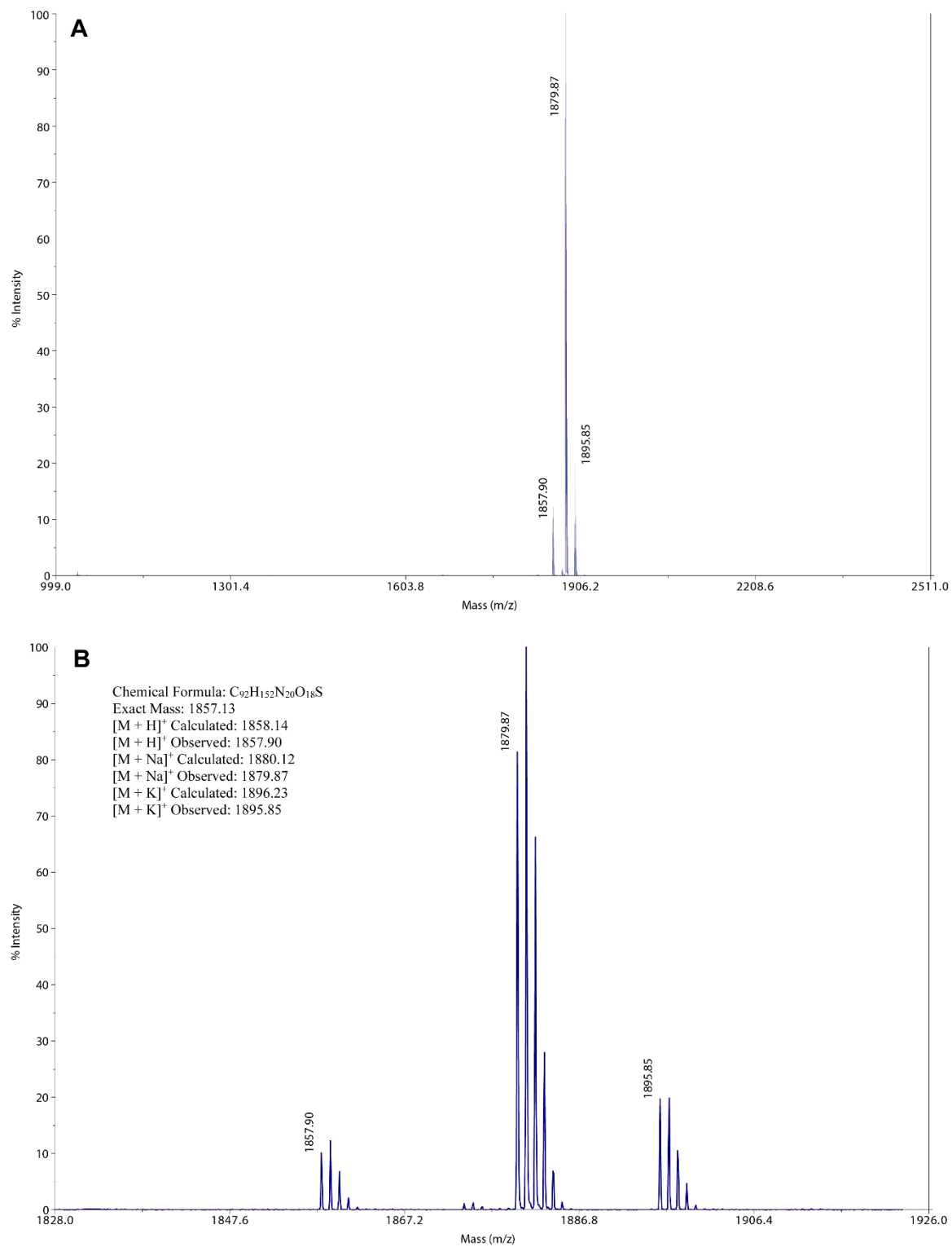
Figure 1.21. MALDI-TOF mass spectrum of peptide 3d . A) Full spectrum. B) Zoomed in spectrum.
