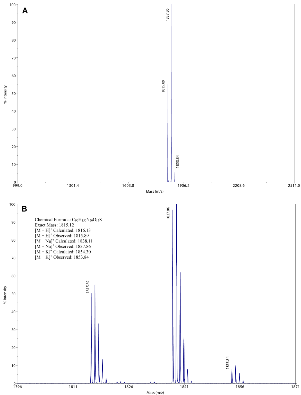
Figure 1.17. MALDI-TOF mass spectrum of peptide 3b . A) Full spectrum. B) Zoomed in spectrum.
