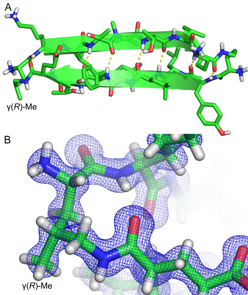
Figure 1.3. (A) X-ray crystallographic structure of peptide 1.1b . (B) 2F o -F c electron density map contoured at the 1 sigma level, showing the conformation of the \delta MeOrn turn unit and the stereochemistry of the \gamma -carbon.
