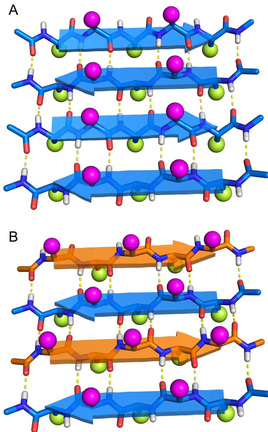
Figure 2.1. Molecular models of (A) pleated \beta -sheets formed from L-peptide strands (blue) and (B) rippled \beta -sheets formed from a mixture of L-peptide and D-peptide strands (orange). Amino acid side chains are depicted as balls, with magenta balls on the top face and yellow balls on the bottom face of the \beta -sheets.
