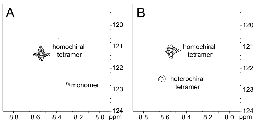
Figure 2.3. ^1\text{H} , ^{15}\text{N} HSQC spectra of (A) 8.0 mM peptide 2.2a and (B) 8.0 mM peptide 2.2a and 8.0 mM peptide ent - 2.1a in 9:1 \text{H}_2\text{O}:\text{D}_2\text{O} at 500 MHz and 298 K.
