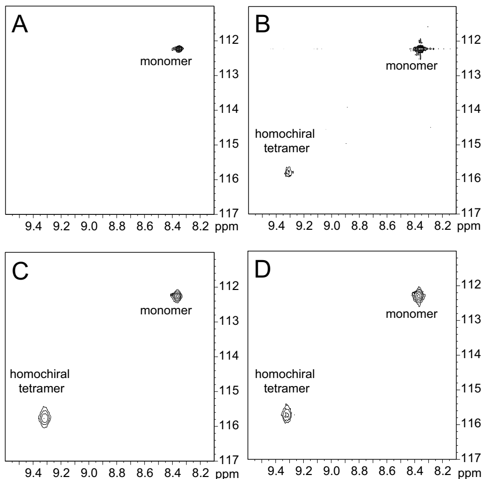
Figure 2.9. ^1\text{H} , ^{15}\text{N} HSQC spectra of (A) 1.0 mM peptide 2.2b , (B) 4.0 mM peptide 2.2b , (C) 8.0 mM peptide 2.2b , and (D) 4.0 mM peptide 2.2b and 4.0 mM peptide ent - 2.1b in 9:1 \text{H}_2\text{O}:\text{D}_2\text{O} at 500 MHz and 298 K.
