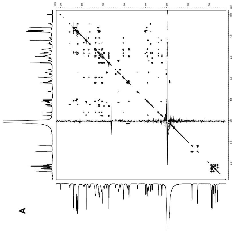
600 MHz TOCSY spectrum of peptide 1.6b 4.0 mM in D 2 O 200-ms spin-lock mixing time, at 277 K
