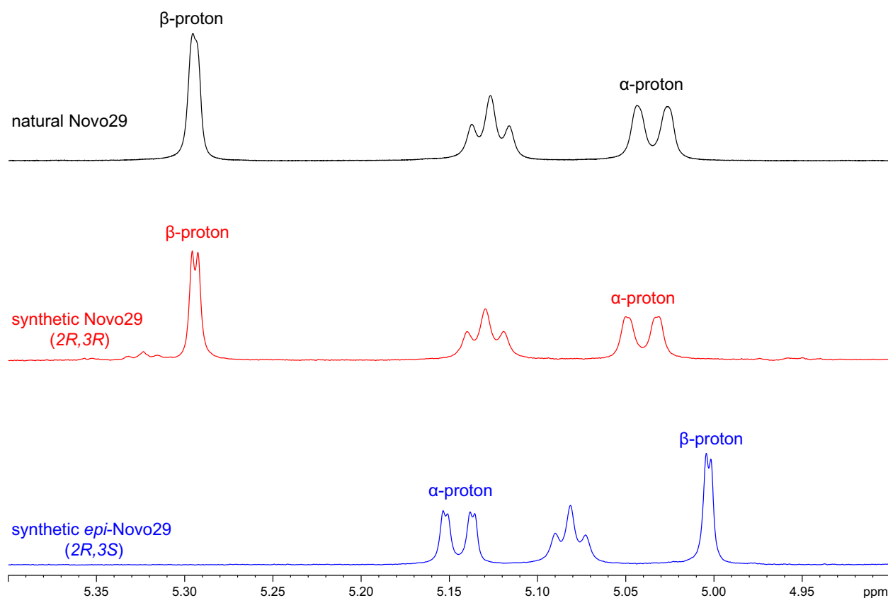
Figure S3.1. Zoom in 1D overlay of natural Novo29 (black), synthetic Novo29 (red), and epi -Novo29 (blue) comparing the \alpha - and \beta -proton chemical shifts of the corresponding hydroxyasparagine. The chemical shifts between natural Novo29 and synthetic Novo29 containing the 2R,3R -hydroxyasparagine match identically, but differ substantially from that of the epi -Novo29.
