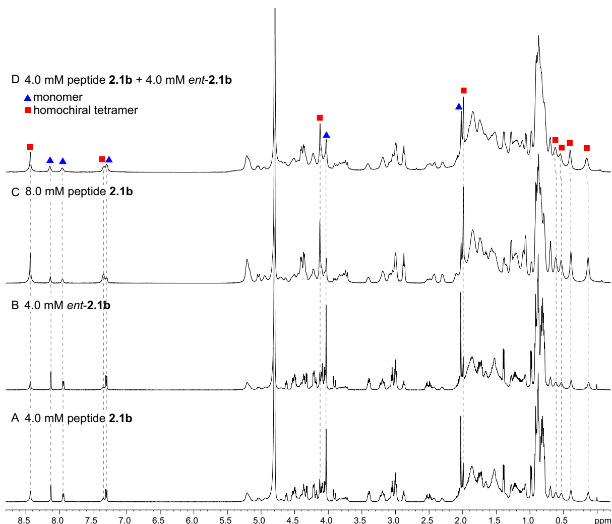
Figure 2.8. ^1\text{H} NMR spectra of (A) 4.0 mM peptide 2.1b , (B) 4.0 mM peptide ent - 2.1b , (C) 8.0 mM peptide 2.1b , and (D) 4.0 mM peptide 2.1b and 4.0 mM peptide ent - 2.1b in \text{D}_2\text{O} at 600 MHz and 298 K with 0.06 mM DSA. 25 (Spectra were referenced against an external DSA standard.) Dashed lines mark key resonances associated with the monomer and homochiral tetramer. These resonances are labeled as follows: blue triangle, monomer; red square, homochiral tetramer.
