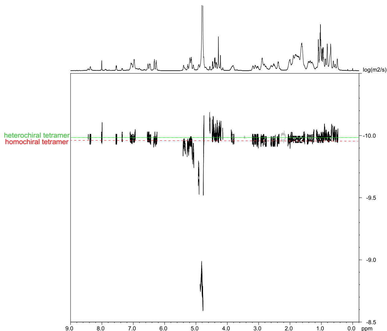
Figure S2.6. DOSY NMR spectrum of 8.0 mM peptide 2.1a and 8.0 mM peptide ent - 2.1a in D 2 O at 600 MHz and 298 K with 0.06 mM DSA 1 . The heterochiral tetramer (green) shows a diffusion coefficient of 10.2 \pm 0.7 \times 10^{-11} \text{ m}^2/\text{s} . The homochiral tetramer (red) shows a diffusion coefficient of 10.7 \pm 0.7 \times 10^{-11} \text{ m}^2/\text{s} . The HOD peak is calibrated to 19.0 \times 10^{-10} \text{ m}^2/\text{s} . 2
