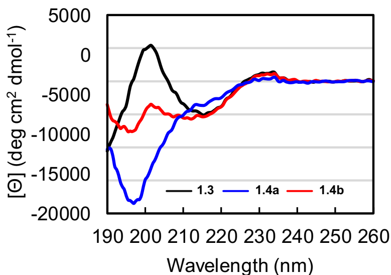
Figure 1.7. CD spectra of peptides 1.3 (black), 1.4a (blue), and 1.4b (red). CD spectra were acquired for each peptide at 100 \mu M in 10 mM phosphate buffer at pH 7.4; the ellipticity was normalized for the number of residues in each peptide.
