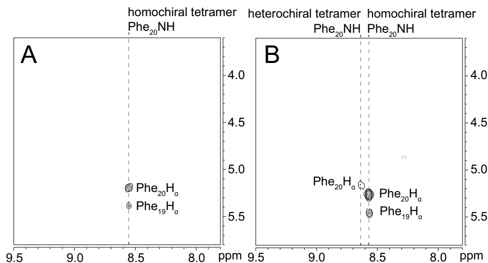
Figure 2.7. ^{15}\text{N} -Edited NOESY spectra of (A) 8.0 mM triply labeled peptide 2.3a and (B) 8.0 mM peptide 2.3a and 8.0 mM unlabeled peptide ent - 2.1a in 9:1 \text{H}_2\text{O}:\text{D}_2\text{O} at 500 MHz and 298 K.
