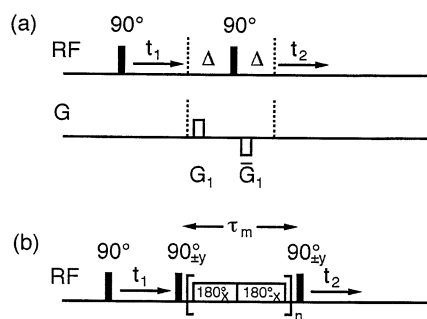
Figure 4. Pulse sequences used in this work. (a) PFG COSY with P-type selection. A fixed delay \Delta=25 ms was used to allow the spectra to be recorded with fewer t_1 increments. The PFGs were 3 \text{ G cm}^{-1} in strength and 1 ms in duration. Connectivities can be quickly determined but coupling constants cannot be measured. (b) Tr-ROESY pulse sequence. The 90^\circ(\pm y) purging pulses allow a phase-sensitive two-dimensional spectrum to be obtained. Throughout the mixing period a train of phase alternating 180^\circ pulses spin locks y-magnetization while inhibiting TOCSY transfer. The RF field strength was 6 kHz during \tau_m . As in conventional ROESY, weak spurious COSY-type cross peaks can arise from zero-quantum coherence.
