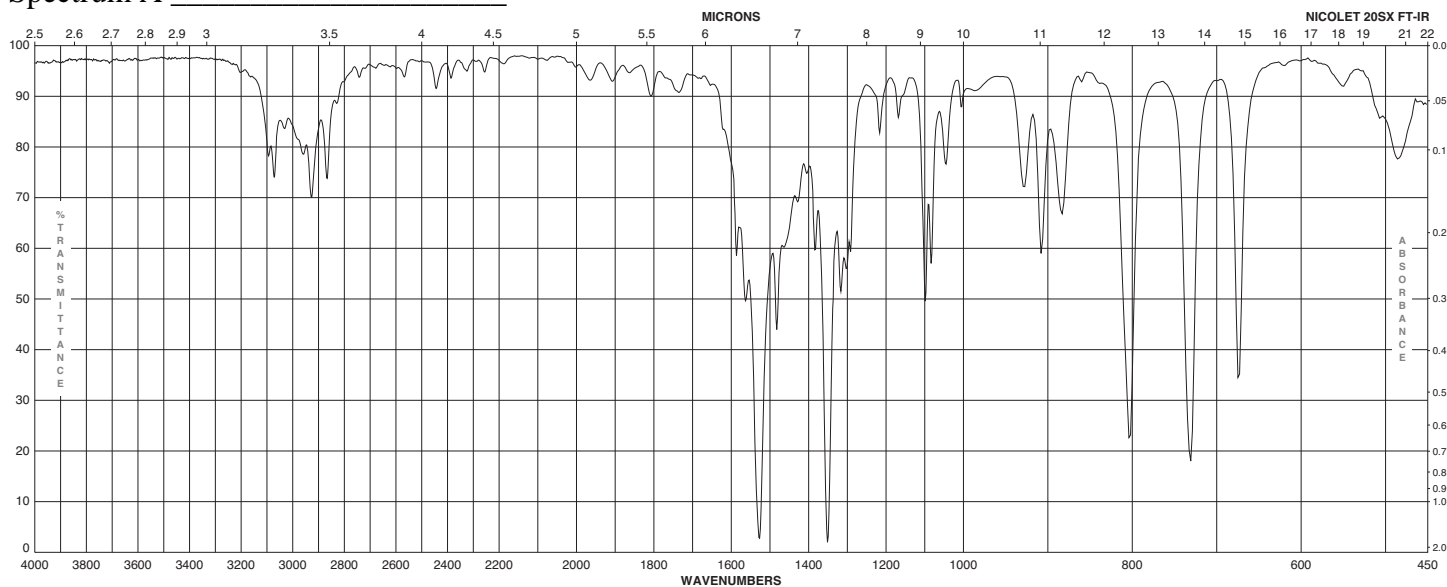
Spectrum A _____
