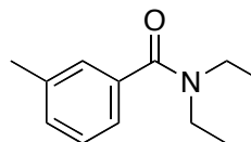
N,N -diethyl- 3-methylbenzamide
