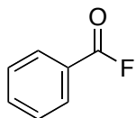
benzoyl fluoride
