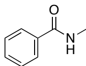
N -methylbenzamide
