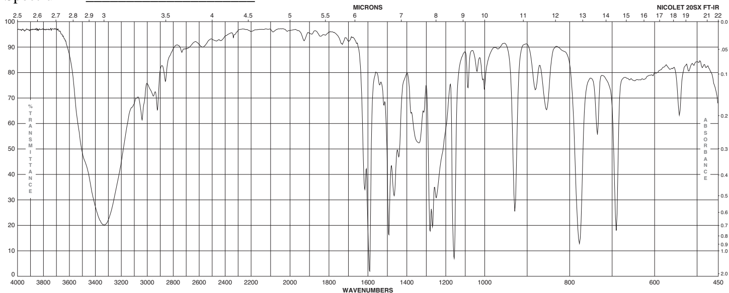
Spectrum A _____
