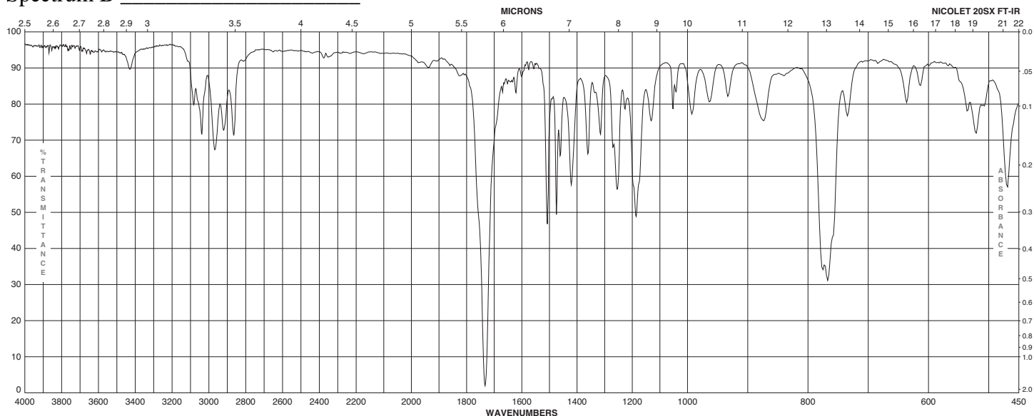
Spectrum B _____
