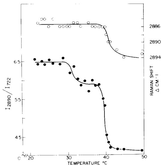
Fig. 8. Melting curve for a dispersion of dipalmitoyl phosphatidylcholine derived from: (1) the change in the intensity ratio I_{2890}/I_{722} (closed circles); (2) change in frequency of the \approx 2890\text{ cm}^{-1} band (open circles).
