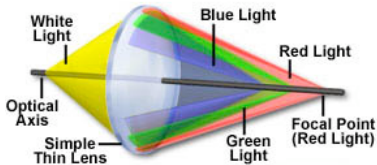
Axial Chromatic Aberration
