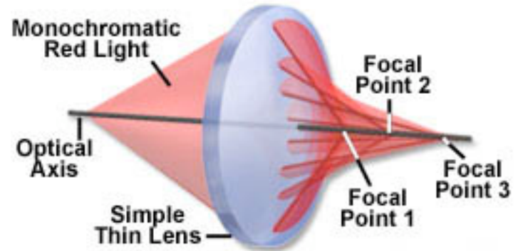
Spherical Aberration
