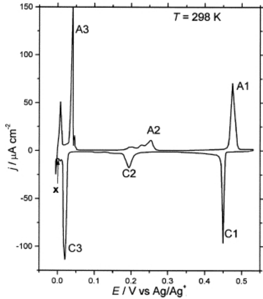
Cyclic voltammogram for Ag upd on Pt(111)( \sqrt{7} \times \sqrt{7} )R19.1°-I.
