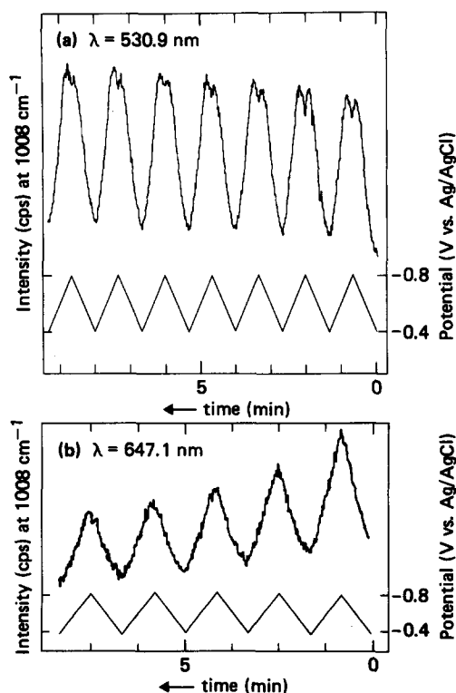
FIG. 4. Irreversible and quasireversible potential dependence of the 1008 \text{ cm}^{-1} ring breathing mode of pyridine. Spectrometer bandwidth: 5 \text{ cm}^{-1} ; (a) laser wavelength 530.9 \text{ nm} ; (b) laser wavelength 647.1 \text{ nm} . See Fig. 2 caption for details of electrochemical system.
