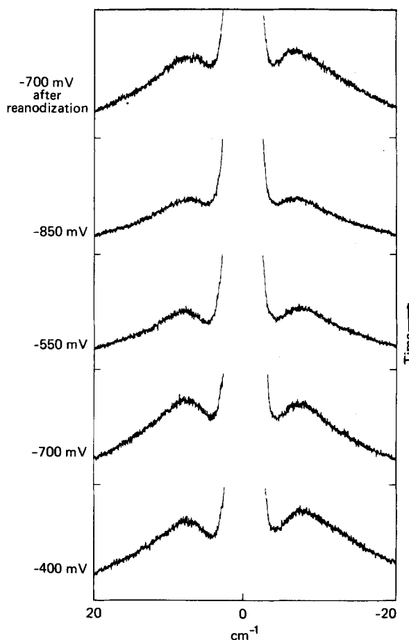
FIG. 2. Low frequency Raman spectra taken sequentially at various electrode potentials following an ORC. Same electrochemical system as in Fig. 1. Laser excitation wavelength: 530.9\text{ nm} . The overall band intensity exhibits a potential dependence which is complicated by an irreversible loss of signal that increases as the electrode potential is swept towards more negative values.
