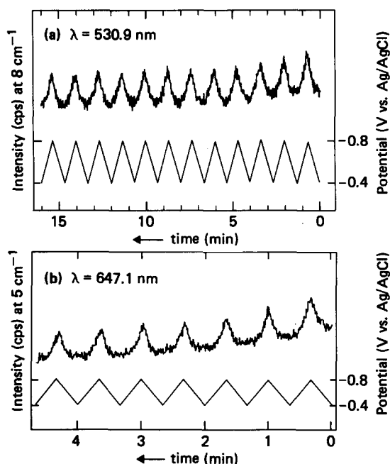
FIG. 3. Irreversible and quasireversible potential dependence of the low frequency Raman bands following an ORC. Same electrochemical system as in Fig. 1. The potential is ramped cyclically from -400 to -800 mV vs Ag/AgCl, starting from the end of the ORC at t = 0 . There is a quasireversible increase of the band intensity with increasingly negative potentials coupled to the irreversible loss of the signal in the same potential range. Spectrometer bandwidth 0.5 \text{ cm}^{-1} . (a) Laser wavelength 530.9 \text{ nm} ; (b) Laser wavelength, 647.1 \text{ nm} .
