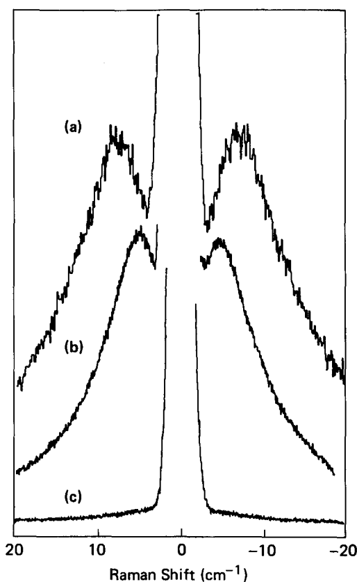
FIG. 1. Low frequency inelastic light scattering from a roughened silver electrode in a 0.1 M KBr + 0.02 M pyridine electrolyte. Incident laser power: 20 mW; resolution: 0.1 cm -1 ; electrode potential: -400 mV vs Ag/AgCl. Curve (a): Stokes and anti-Stokes Raman scattering after the electrode was polarized to -1400 mV for 10 s and then subjected to an ORC which delivered 25 mC/cm 2 to the electrode; laser wavelength: 530.9 nm. Curve (b): same as curve (a) except with a laser wavelength of 647.1 nm. Curve (c): same as curve (a) except that the electrode potential was held at -1400 mV for 5 s after the ORC.
