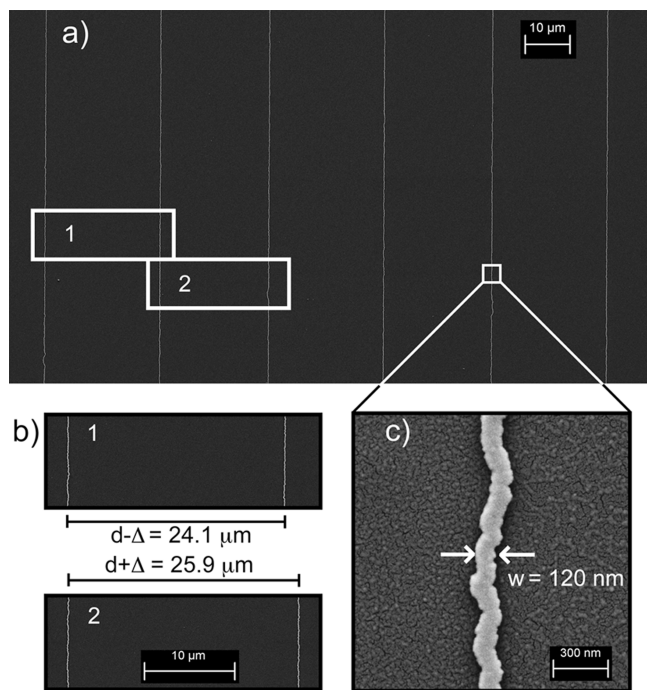
Figure 2. SEM images of an Au nanowire grating: (a) large area scan showing average wire spacing of 25\ \mu\text{m} . (b) Overlaying images of a neighboring nanowire pair revealing asymmetry due to the etching and growing steps where d - \Delta = 24.1\ \mu\text{m} , d + \Delta = 25.9\ \mu\text{m} . (c) High-magnification image of a single Au nanowire with w = 120\ \text{nm} .
