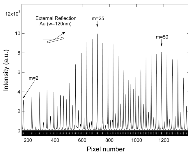
Figure 9. External reflection geometry line profile of the diffraction pattern of an Au nanowire grating with w = 120 nm and \Delta/d = 4.0\% . Beneath is the image used to obtain the line profile with enhanced contrast to easily visualize the diffraction spots.
