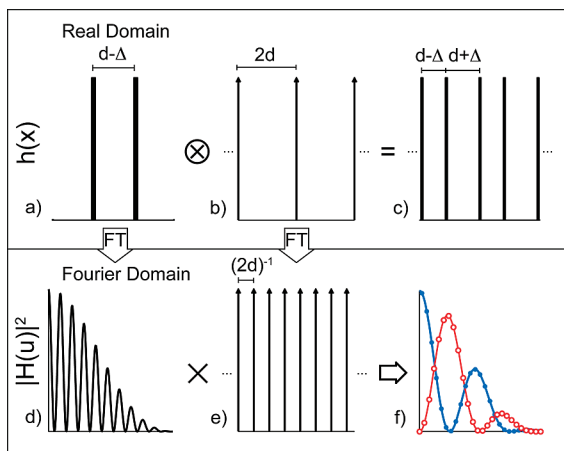
Figure 7. Schematic diagram of the convolution theorem analysis involved in finding the diffraction pattern of a particular grating. The grating is modeled in the real domain: (a) an asymmetric grating unit cell formed by two square pulses is convolved with (b) a Dirac comb of spacing 2d to yield (c) an infinite asymmetric grating. The diffraction pattern is found in the Fourier domain: (d) The FT of the unit cell (plotted as the |H(u)|^2 ) is multiplied by (e) the FT of the Dirac comb. The square magnitude of each integrated peak is taken to yield (f) the predicted diffraction pattern, where the solid blue dots are the even orders and open red dots are the odd orders. The solid lines in Figure 7f are the intensity functions for the even and odd orders (see eqs 3 and 4).
