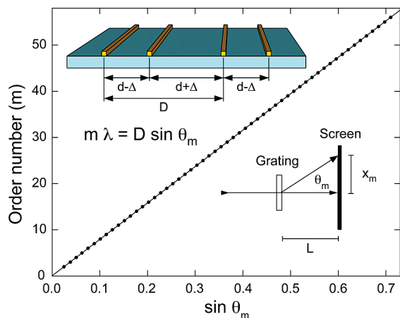
Figure 5. Plot of experimentally determined order number ( m ) versus \sin \theta_m as defined by the bottom inset where each dot represents one order. The solid line is the fit as predicted by the grating equation (eq 2). A zero intercept ensures the orders number were assigned correctly and the slope of the line is D/\lambda , where D = 50.2 \pm 0.1 \mu\text{m} . The top inset shows how the asymmetry forces the grating period D = 2d .
