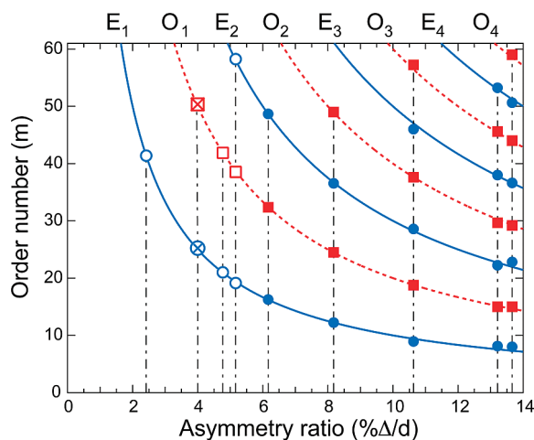
Figure 8. Plot of the order of occurrence of even ( E_n , solid curves) and odd ( O_n , dashed curves) minima versus the percent asymmetry ratio as predicted by eqs 5 and 6. Vertical dashed–dotted lines represent each sample with circles as their even minima and squares as their odd minima. Six Au (solid) and three Pd (open) grating diffraction patterns are fit to the curves to determine their asymmetry ratio, \Delta/d . The Au sample from Figure 6 is depicted by the open-crossed symbols at \Delta/d = 4.0\% .
