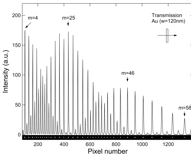
Figure 4. Transmission geometry line profile of the diffraction pattern of an Au nanowire grating with w = 120\ \text{nm} and \Delta/d = 4.0\% , displaying orders from m = 3 to 59 . Beneath is the image used to obtain the line profile with enhanced contrast to easily visualize the diffraction spots.
