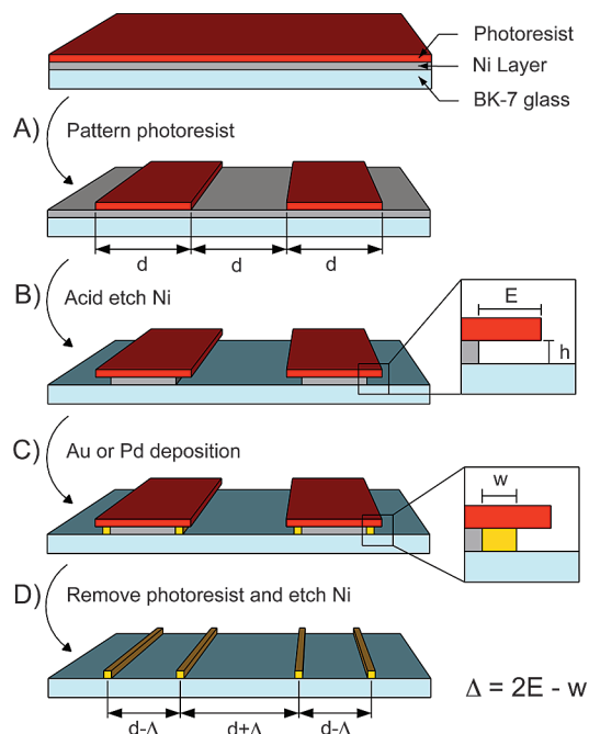
Figure 1. Schematic flow diagram of the LPNE process for fabrication of either Au or Pd nanowire gratings with nanowire height h of 45 nm, width w of 25–150 nm, and alternating interwire spacing d - \Delta and d + \Delta , where d is 25 \mu\text{m} and \Delta is a deviation from symmetry varying from 0 to 3.5 \mu\text{m} due to the asymmetric etching depth E and growing as defined in the figure. See text for details.
