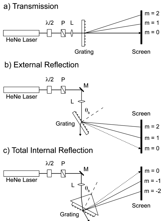
Figure 3. Schematic diagram of the three geometries used to obtain diffraction images. In all cases, the source is a HeNe laser with a polarizer (P) and a \lambda/2 plate to control the intensity and final polarization, and a lens (L) to focus the image on the screen. (a) In the transmission geometry, the laser impinges normal to the surface. (b) In the external reflection and (c) total internal reflection geometries, the laser impinges at Brewster's angle ( \theta_b ) for an air–glass and glass–air interface, respectively.
