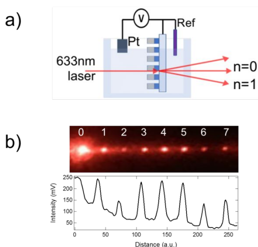
18 19 20 21 22 23 24 25 26 27 28 29 30 31 32 33 34 Figure 4. a) Schematic of the setup used for electrochemically modulated optical measurements 35 of ZnO-WO 3 and ZnO-PEDOT gratings. b) Photograph of and intensity profile of diffraction 36 pattern created by a set of ZnO-WO 3 gratings.
