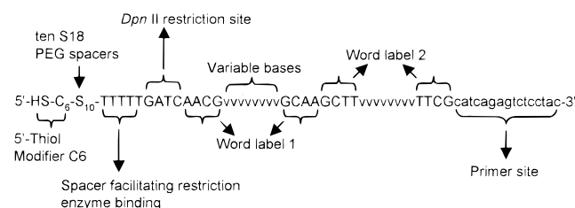
Figure 2. Sequence design of the surface-bound multiple-word oligonucleotides. 5'-HS-C6 is 5'-thiol-modifier C6 which reacts with the maleimide-functionalized gold surfaces; S 10 corresponds to ten S18 PEG spacers, which separate the hybridizing sequence from the solid support; GATC is the recognition site for the restriction enzyme Dpn II; TTTT is inserted here as a spacer to enhance the efficiency of the restriction enzyme cleavage step. This reflects the fact that additional bases flanking restriction enzyme recognition sites are often required when the cleavage occurs close to the end of the double-stranded DNA substrate being cleaved. 32 AACG...GCAA and GCTT...TTCG sequences are the “word labels” used to target hybridization to a particular word, and the variable sequence denoted by “vvvvvvv” is used to encode information. “catcagagtctctac” is a primer site for the polymerase extension reaction. The primer sequence employed was 5'-6-FAM-gtaggagactctgatg 3'.
